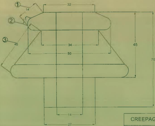
UPPER INSULATOR
